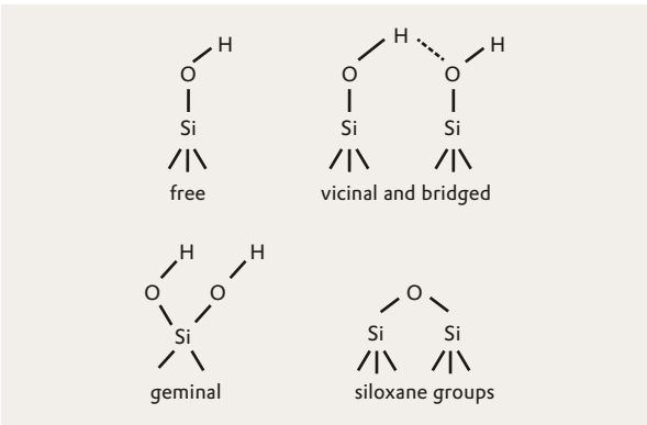
Figure 4 - Surface chemistry
